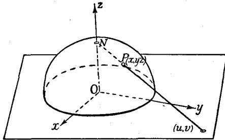
Fig. 14.—Stereographic projection of the sphere
