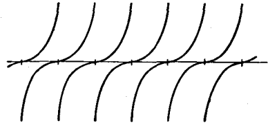
Fig. 28.—Family of cubical parabolas
