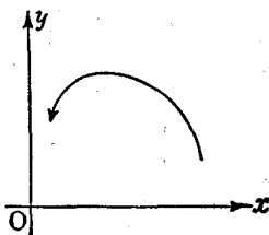
Fig. 2.—Right-handed system of axes
