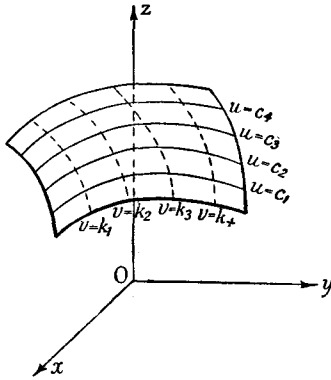
Fig. 17.—Parametric curves u = \text{const.} , v = \text{const.}
