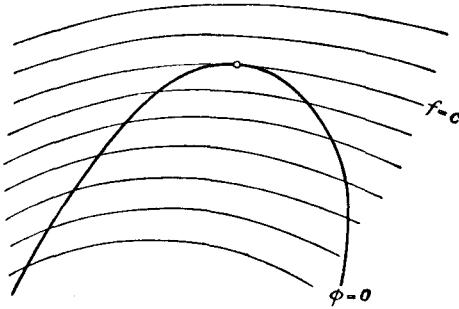
Fig. 30.—Extreme value of f with subsidiary condition \phi = 0
