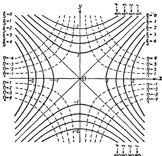
Fig. 8.—Orthogonal families of rectangular hyperbolas
