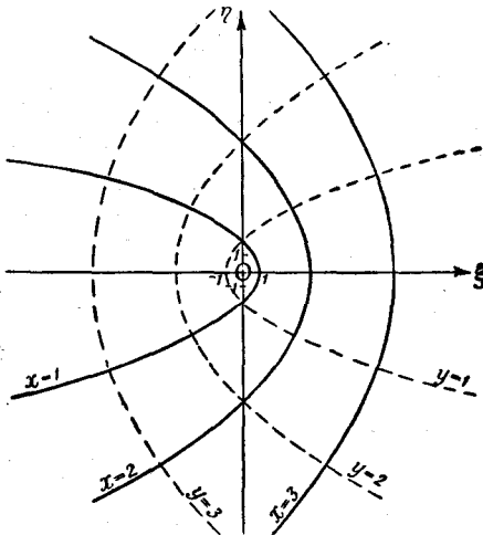
Fig. 9.—Orthogonal families of confocal parabolas
