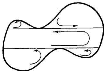
Fig. 5.—Non-convex region formed from convex regions
