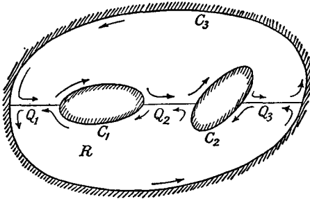
Fig. 3.—A multiply-connected region R subdivided by Q_1, Q_2, \dots into simply-connected regions
