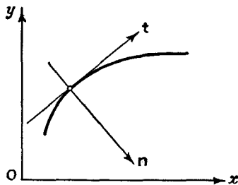
Fig. 6.—Tangent and normal directions
