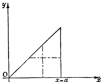
Fig. 8.—Triangle as region of integration
