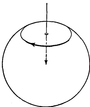
Fig. 10.—Positively oriented sphere
