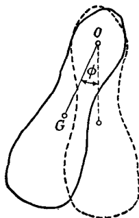
Fig. 14.—The compound pendulum
