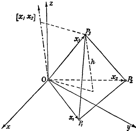
Fig. 17.—Determination of the volume of a tetrahedron
