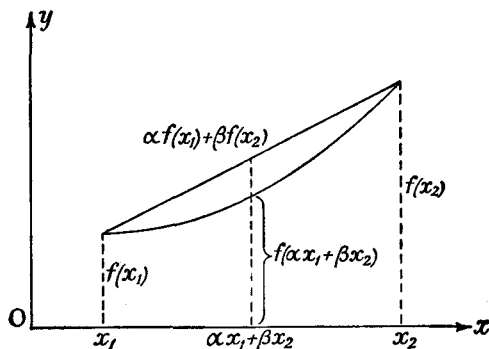
Fig. 19.—A function which is convex downwards
