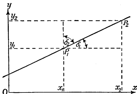
Fig. 11.—Parametric representation of a straight line passing through two points
