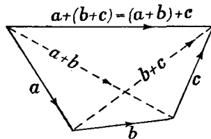
Fig. 9.—Associative law of vector addition
