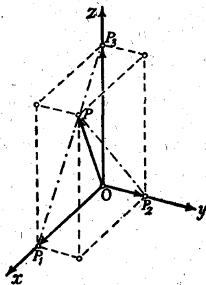
Fig. 1.—Co-ordinate axes in space
