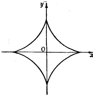
Fig. 23.—Astroid
