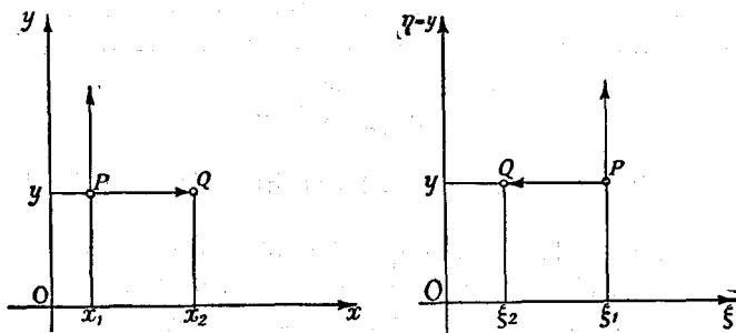
Fig. 13.—Transformation in which the sense of rotation is reversed
