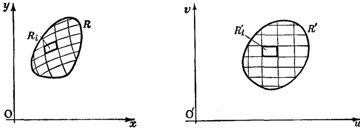
Figs. 9, 10.—Decomposition of regions in a transformation
