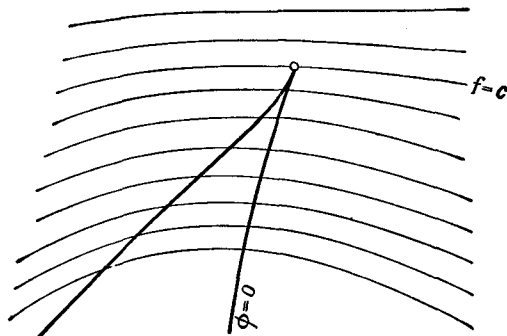
Fig. 31.—Extreme value at a singular point of \phi = 0
