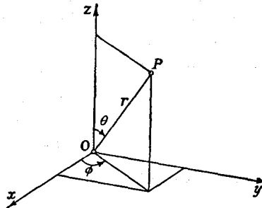
Fig. 10.—Three-dimensional polar co-ordinates
