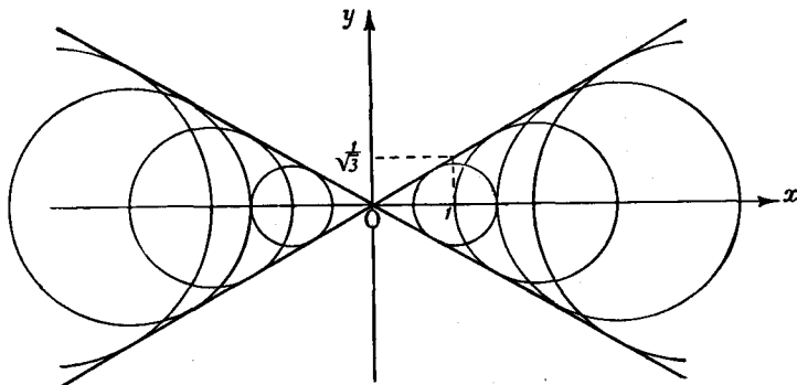
Fig. 21.—The family (x - 2c)^2 + y^2 - c^2 = 0
