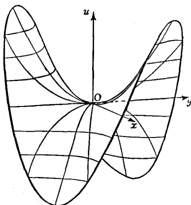
Fig. 1.—The surface u = xy
