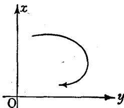
Fig. 3.—Left-handed system of axes
