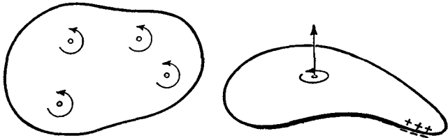
Fig. 8.—Orientation of a curved surface
