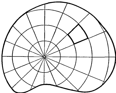
Fig. 3.—Subdivision by polar co-ordinate nets
