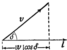
Fig. 7.—Projection of a vector
