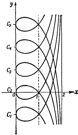
Fig. 27.—Family of strophoids
