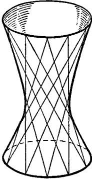
Fig. 15.—Hyperboloid of one sheet
