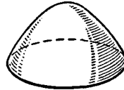
Fig. 16.—Hyperboloid of two sheets
