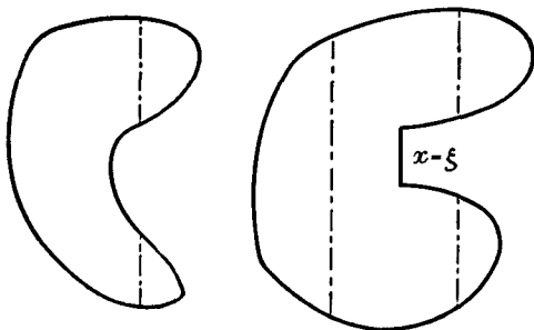
Fig. 6.—Non-convex regions of integration
