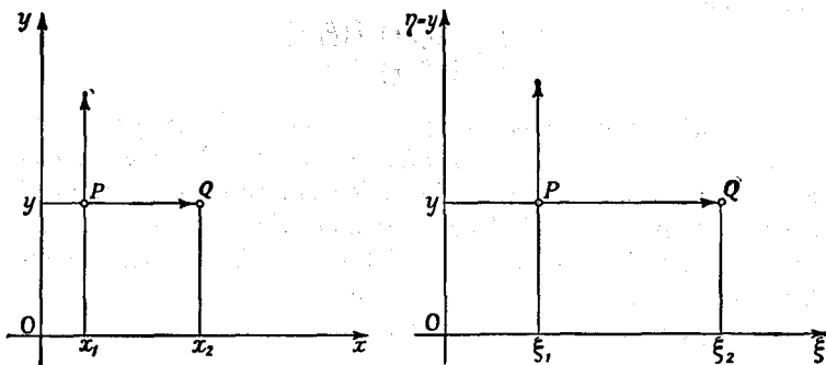
Fig. 12.—Transformation in which the sense of rotation is preserved
