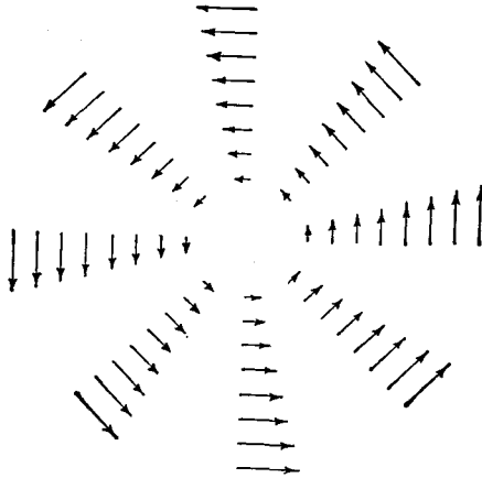
Fig. 8.—The velocity field in a rotation
