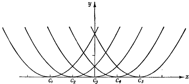
Fig. 20.—Family of parabolas with envelope
