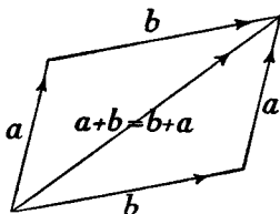
Fig. 8.—Commutative law of vector addition
