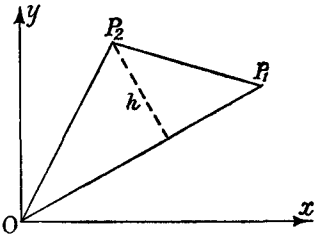
Fig. 12.—To illustrate the method for finding the area of a triangle
