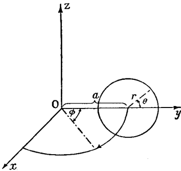
Fig. 18.—Generation of an anchor ring by the rotation of a circle
