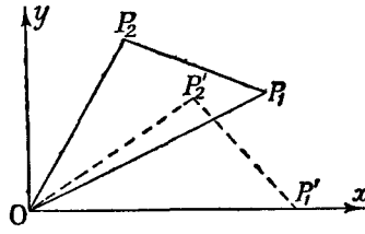
Fig. 13.—Determination of the sign of the area of a triangle
