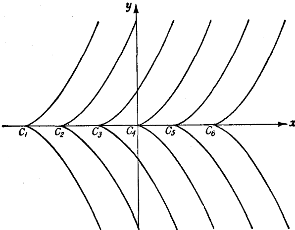
Fig. 26.—The family (x - c)^3 - y^2 = 0
