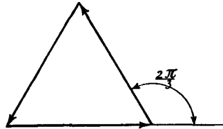
Fig. 29.—Three vectors with equal magnitudes and sum zero
