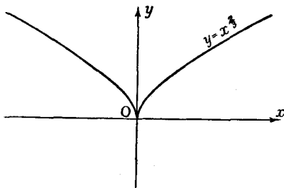
Fig. 5.—The surface y^3 - x^2 = 0
