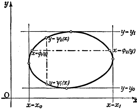
Fig. 4.—General convex region of integration
