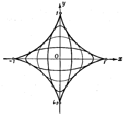
Fig. 24.—Astroid as envelope of ellipses
