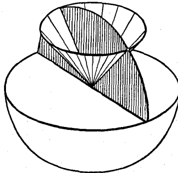
Fig. 11.—Co-ordinate surfaces for three-dimensional polar co-ordinates
