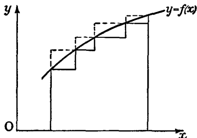
Fig. 15.—Approximation to a region by sets of rectangles
