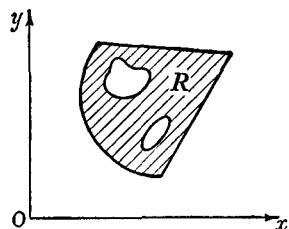
Fig. 2.—A triply-connected region
