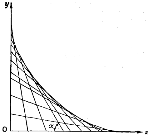
Fig. 22.—Arc of the astroid as envelope of straight lines
