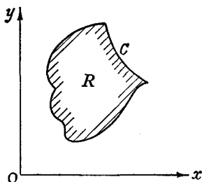
Fig. 1.—A simply-connected region
