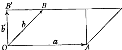
Fig. 15.—To show that [ab] = [ab']
