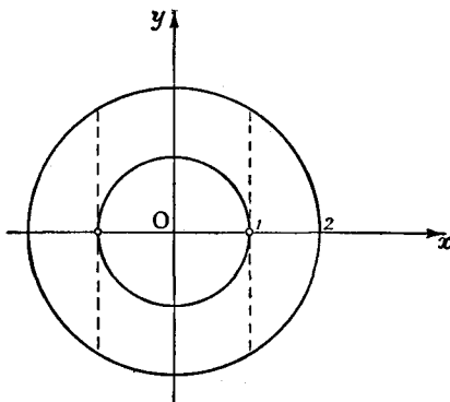
Fig. 7.—Circular ring as region of integration
