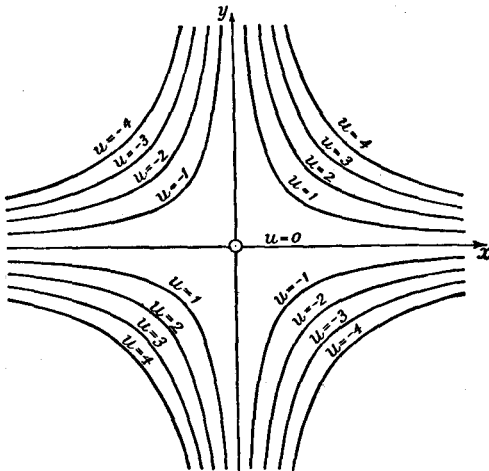
Fig. 2.—Contour lines of u = xy
