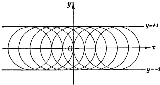
Fig. 19.—Family of circles with envelope
