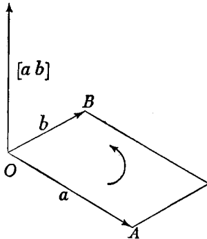
Fig. 14.—Vector product of two vectors a and b
