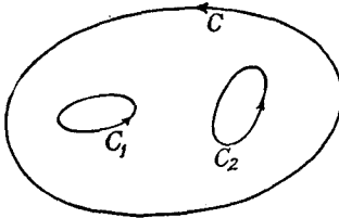
Fig. 2.— \int_{\sigma} = \int_{\sigma_1} + \int_{\sigma_2}
