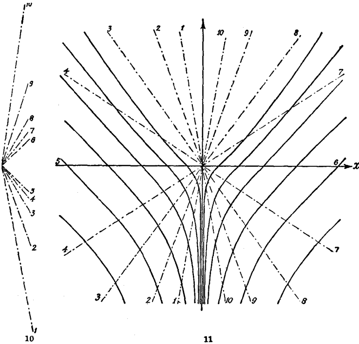
Fig. 10.—Directions of the integral curves on the isoclines in fig. 11
