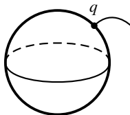
Fig. 5.7. Sphere with a hair.
