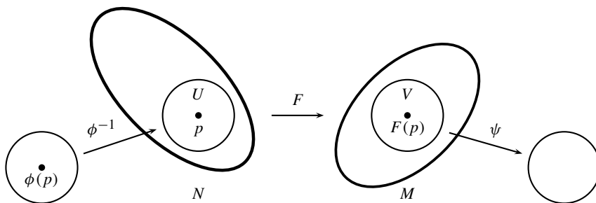
Fig. 6.3. Checking that a map F : N \rightarrow M is C^\infty at p .
