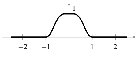
Fig. 13.1. A bump function at 0.
