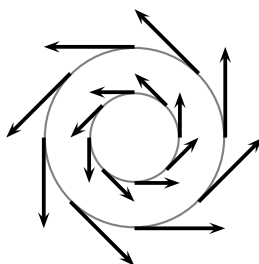
Fig. 12.3. The vector field (-y, x) in \mathbb{R}^2 .
