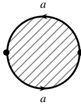
Fig. 27.9. The real projective plane.
